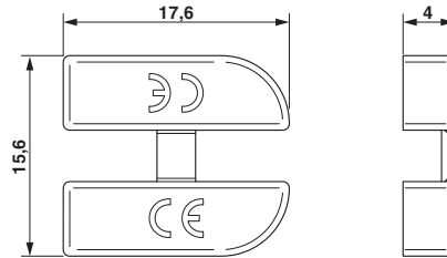
Dimensional drawing
